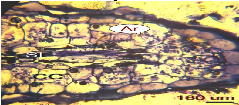
Fig.1A, 1B and 1C: Feeder root of Eucalyptus camaldulensis , Casuarina glauca and A. salign infected with AM fungus. V: vesicle, H: internal hyphae of the fungus, CC: cortex cells, St: stele and Ar: arbuscule.
