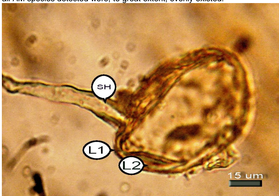
Fig. 3: Clamydospore of Glomus aggregatum . L1 and L2 is the outer and inner spore wall, respectively and SH is the subtending hyphae.
