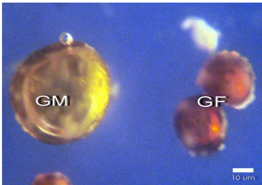
Fig. 4: Stereo shape of the chytrid spore of Glomus mossae (GM) and G. fasciculatum .
