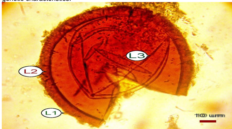
Fig. 5: Chytrid spore of Glomus fasciculatum . L1, L2 and L3 is the outer, middle and inner spore wall, respectively.
