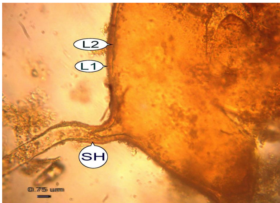
Fig. 6: Clamydospore of Glomus mossae . L1 and L2 is the outer and inner spore wall, respectively and SH is the subtending hyphae.
