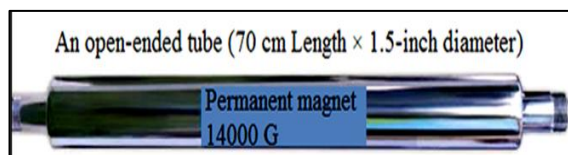
Fig. 1. The permanent magnet instrument used for the pre-sowing MT of barley seeds.
