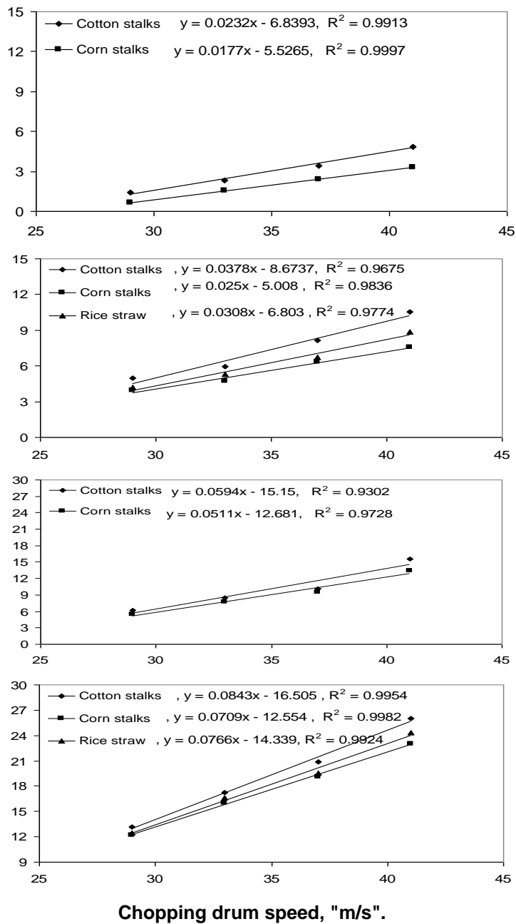
Fig. (7): The effect of chopping drum speed, "m/s" on the power requirements, "kW" before and after machine modification.
