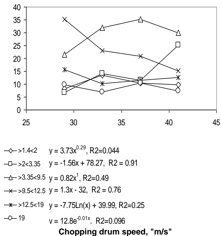
Fig. (8): The effect of chopping drum speed, "m/s" on cutting lengths, "%", before machine modification.
