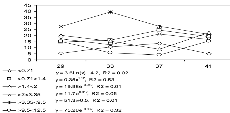
Fig. (9): The effect of chopping drum speed, "m/s" on cutting lengths, "%", after machine modification.
