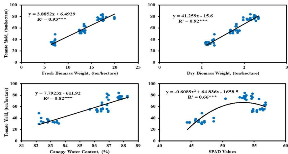
Fig. 8. Relationship between Tomato Yield (ton/ha) and FB (ton/ha), DB (ton/ha), CWC (%), and SPAD values during combined data from Both Seasons
