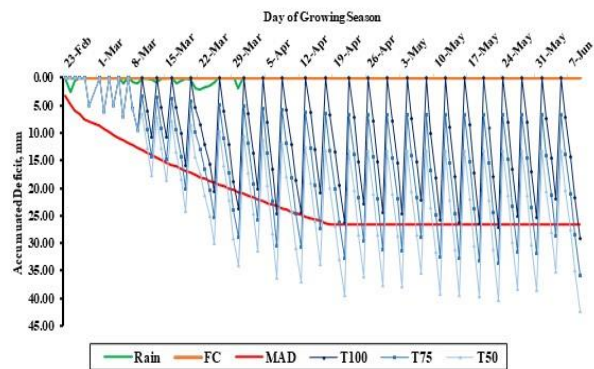
Fig. 4. Tomato crop irrigation scheduling for 2022 season at different irrigation treatments
