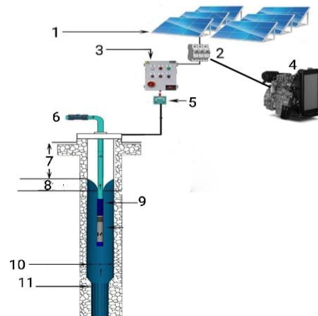
1. PV module 2. DC breaker 3. Control box 4. Engine 5. Switch 6. Water output 7. Static water level 8. Drawdown 9. Pump 10. Well diameter 11. Strainer Fig. 3. Hybrid energy sources (HES)
