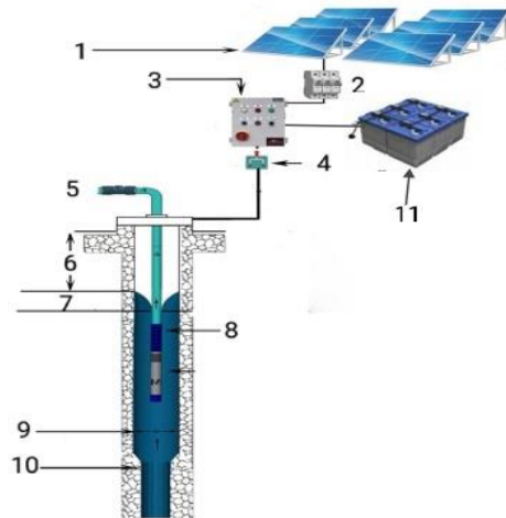
1- PV module 2- DC breaker 3- Control box 4-Switch 5- Water output 6- Static water level 7- Drawdown 8. Pump 9. Well diameter 10- Strainer 11-Batteries Fig. 2. Solar Photovoltaic System (PVS)
