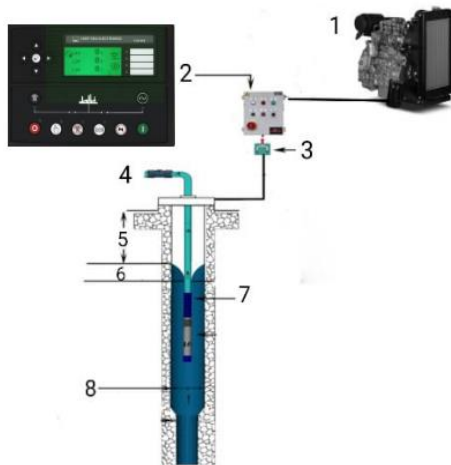
1- Diesel engine 2-Control box 3- Switch 4- Water output 5-Static water level 6. Drawdown 7. Pump 8-Well diameter Fig. 1. Petrol Power System (PPS) connecting with the water well
