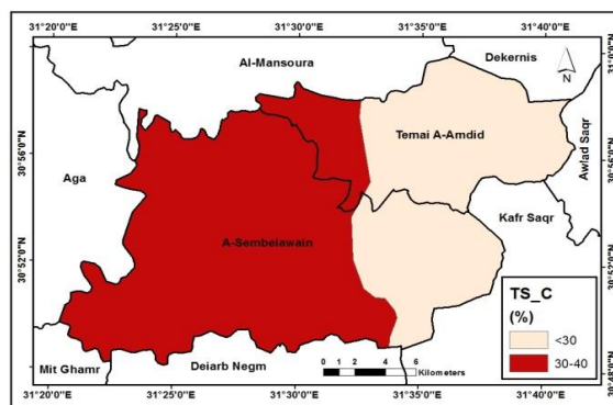
Figure 2. Spatial variability within total sand (TS) at the subsurface layer (60-90 cm) of the studied soils.
